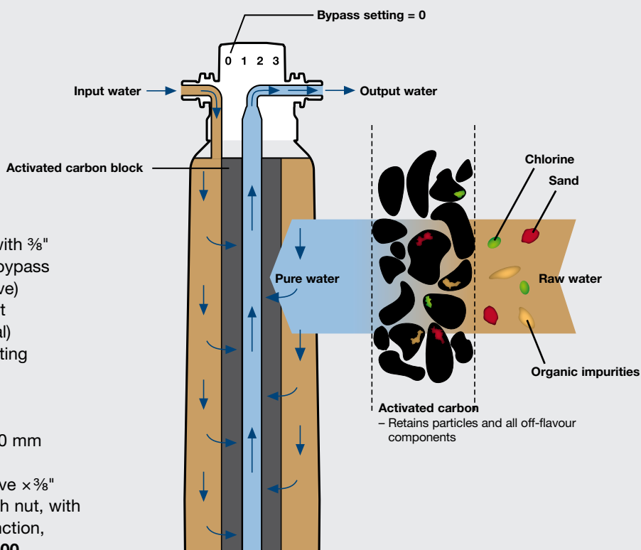
Layout of a besttaste filter cartridge
